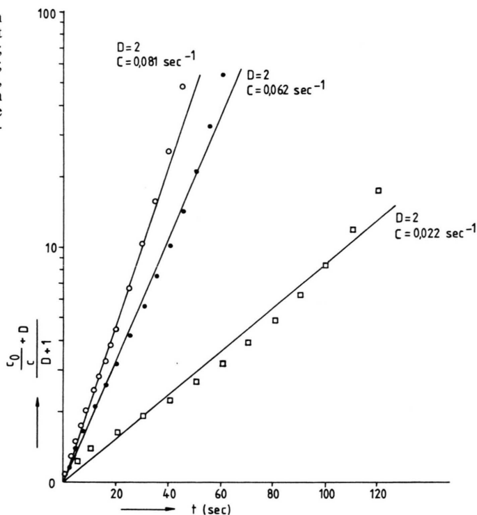
Fig. 7. Kinetics of the back reaction in Chlorella in the presence of DCMU and 750 mM \text{NH}_4\text{Cl} at various pH values. \circ pH = 6.5; \bullet pH = 7.0; \square pH = 7.5. Phosphate buffer; T = 25^\circ\text{C} ; DCMU, 20 \mu\text{M} ; Chl, 42 \mu\text{g}/\text{ml} . Preillumination time, 30 sec. Kinetic data are represented as indicated in the section "Theoretical concepts". C_0 and C denote the maximal concentration of \text{Q}^- or its concentration at time t , respectively.
